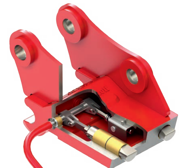
Socket wrench turned 120°, quickcoupler securely locked over dead center
